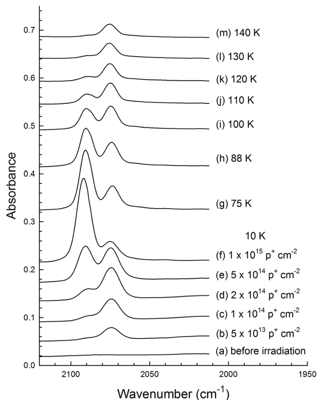
Fig. 5 Infrared spectra of acetic acid- 1\text{-}^{13}\text{C} , before and after irradiation at 10 K, (a)–(f), showing the growth of ^{13}\text{CO} and \text{H}_2\text{C}=\text{C}=\text{O} . Traces (g)–(m) show the effect of warming the irradiated ice. The proton fluences were as given in the figure. The ice's original thickness was about 1.0\ \mu\text{m} . Spectra have been offset for clarity.
