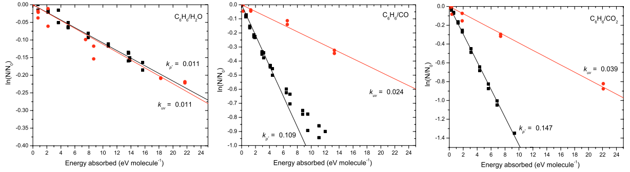
Fig. 8. Destruction of benzene in: water ice (1:5, left panel ), in CO (1:30, middle panel ) and in CO 2 (1:20, right panel ) ices as a function of absorbed energy dose (● = UV, ■ = protons). The negative slope ( k ) of the plot is related to destruction cross section and half-life through Eqs. (7)-(9).
