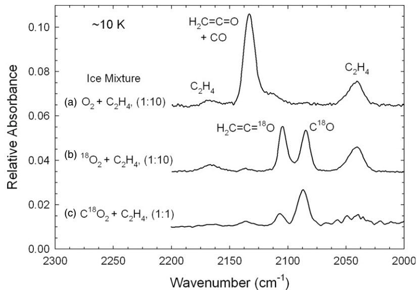
Figure 7. Spectra showing the formation of ketene in irradiated ethylene-containing ices. The formation of ^{18}\text{O} -labeled ketene (left) and CO (right) are shown. Ion fluences are approximately (a) 1 \times 10^{14} p^+ \text{ cm}^{-2} , (b) 1 \times 10^{14} p^+ \text{ cm}^{-2} , and (c) 2 \times 10^{14} p^+ \text{ cm}^{-2} .
