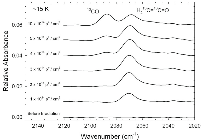
Figure 6. Spectra of \text{H}_2\text{O} + {}^{13}\text{C}_2\text{H}_2 (5:1) after various stages of proton irradiation (bottom to top). The formation of {}^{13}\text{C} -labeled ketene (right) and CO (left) are shown.
