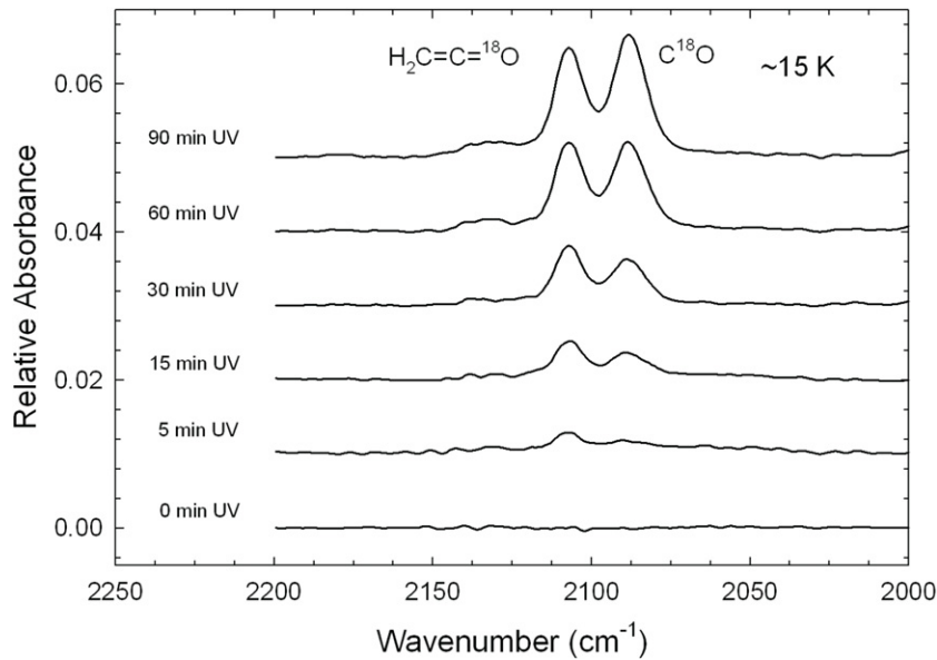
Figure 3. Spectra showing ^{18}\text{O}_2 + \text{C}_2\text{H}_2 (1:1) at \sim 15 K after various stages of UV photolysis (bottom to top).
