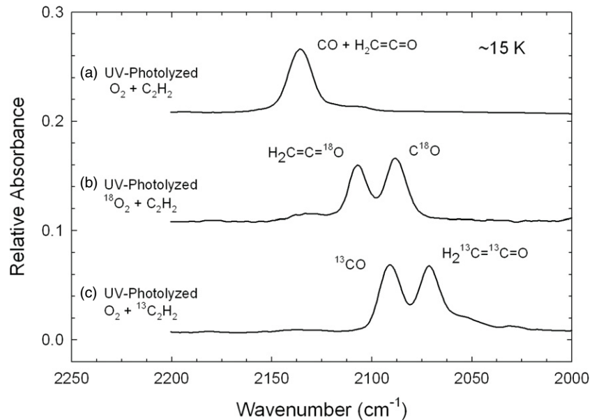
Figure 2. Spectra of the UV photolysis (90 minutes) at \sim 15 K of \text{O}_2 + \text{C}_2\text{H}_2 ices, showing formation of ketene ( \text{H}_2\text{CCO} ) and CO. The ices initially were composed of (a) \text{O}_2 + \text{C}_2\text{H}_2 , (b) ^{18}\text{O}_2 + \text{C}_2\text{H}_2 , and (c) \text{O}_2 + ^{13}\text{C}_2\text{H}_2 . No IR features were present in this region before photolysis of the samples. In each case, the initial ice composition was \text{O}_2:\text{C}_2\text{H}_2 \approx 1:1 .
