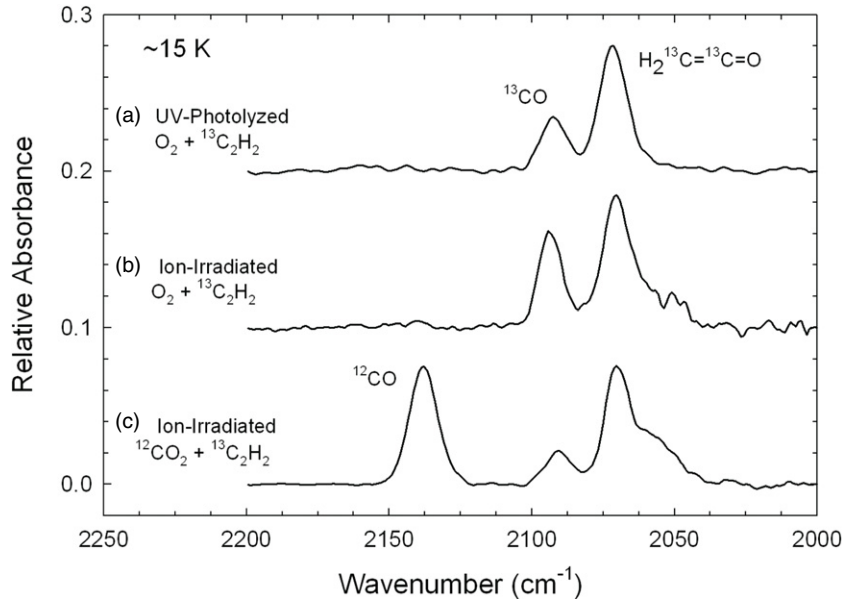
Figure 4. Spectra showing the similarity of reaction products from UV photolysis and proton irradiation, and from \text{O}_2 and \text{CO}_2 as sources of oxygen: (a) \text{O}_2 + ^{13}\text{C}_2\text{H}_2 after 5 minute UV photolysis, (b) \text{O}_2 + ^{13}\text{C}_2\text{H}_2 after 2 \times 10^{13} p^+ \text{cm}^{-2} , and (c) \text{CO}_2 + ^{13}\text{C}_2\text{H}_2 after 1 \times 10^{14} p^+ \text{cm}^{-2} , with each ice initially being a 1:1 mixture.
