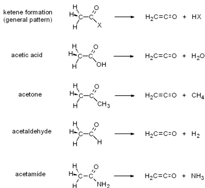
Figure 8. Experiments have shown that the four interstellar molecules named on the left can decompose to give ketene. See the Introduction for references. Solid wedges represent chemical bonds coming out of the plane of the drawing and toward the reader, while dashed wedges represent chemical bonds going behind the plane of the drawing and away from the reader.
