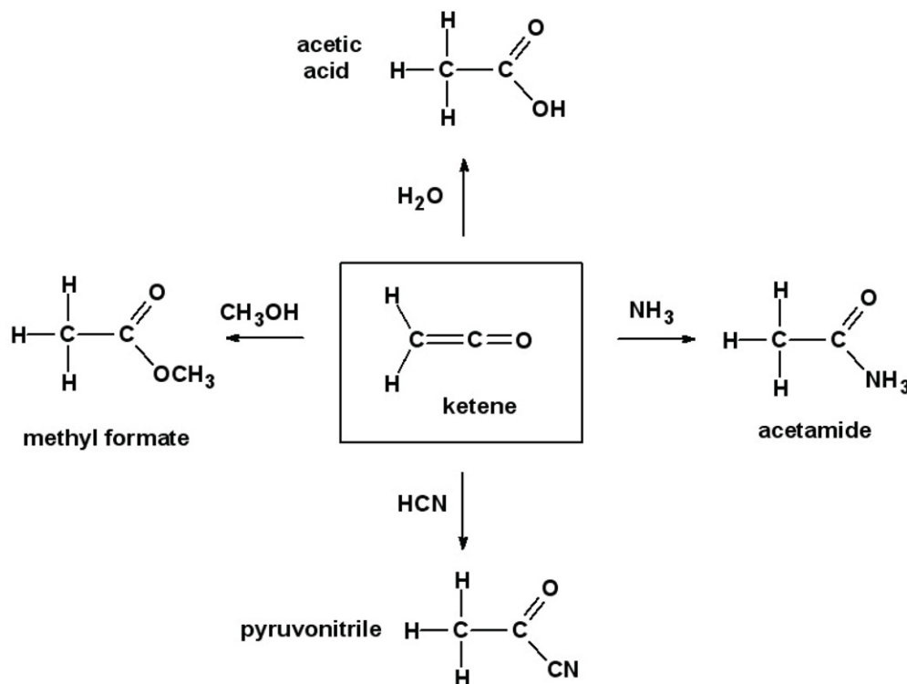
Figure 1. Four laboratory addition reactions of ketene. See Staudinger (1912), Wang & Schueler (1949), Quadbeck (1956), and references therein for details.
