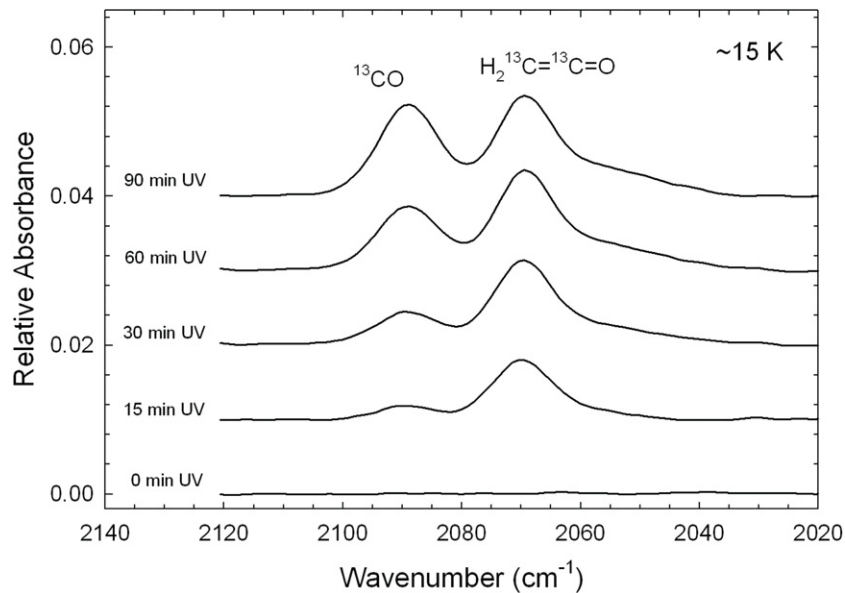
Figure 5. Spectra of \text{H}_2\text{O} + {}^{13}\text{C}_2\text{H}_2 (5:1) at \sim 15 K after various stages of UV photolysis (bottom to top). The formation of {}^{13}\text{C} -labeled CO (left) and ketene (right) are shown.
