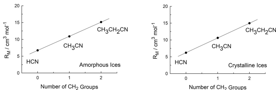
Fig. 6. Molar refractions of three organic compounds. The left-hand plot is for amorphous ices and the right-hand plot is for crystalline ices. See Table 1 for the n and \rho values used to calculate R_M .
