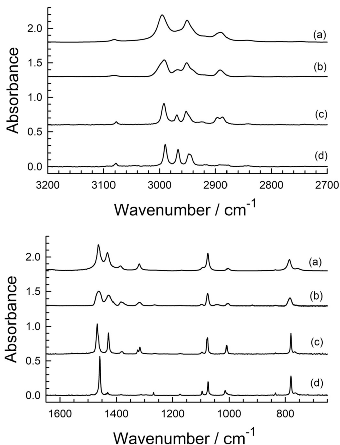
Fig. 5. Expansions of IR spectra of \text{CH}_3\text{CH}_2\text{CN} . See the caption of Fig. 4 for details.
