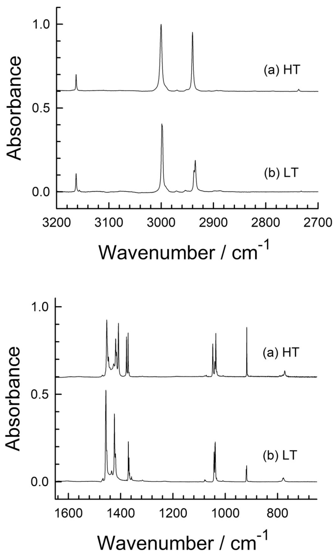
Fig. 2. Expansions of IR spectra of \text{CH}_3\text{CN} . See the caption of Fig. 1 for details.
