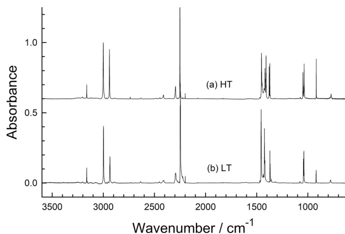
Fig. 1. Survey spectra of two crystalline forms of \text{CH}_3\text{CN} at 120\text{ K} . (a) The sample was deposited at 120\text{ K} , warmed to 150\text{ K} , and cooled to 120\text{ K} to give the high-temperature (HT) crystalline phase. (b) The sample was deposited at 10\text{ K} , warmed to 165\text{ K} , and cooled to 120\text{ K} to give the low-temperature (LT) crystalline phase. Spectra have been offset for clarity. Note that the peak near 2245\text{ cm}^{-1} is off-scale in each spectrum, so as to show the weaker features. The spectral resolution was 0.5\text{ cm}^{-1} .
