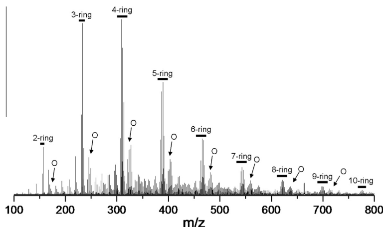
Fig. 3. APPI mass spectrum of the residue made from benzene irradiated at 19 K by 0.8 MeV protons. Polyphenyls and partially hydrogenated polyphenyls up to 10-ring compounds are indicated by the horizontal lines. Mass envelopes of oxygenated species also are present, and are marked by “O”.
