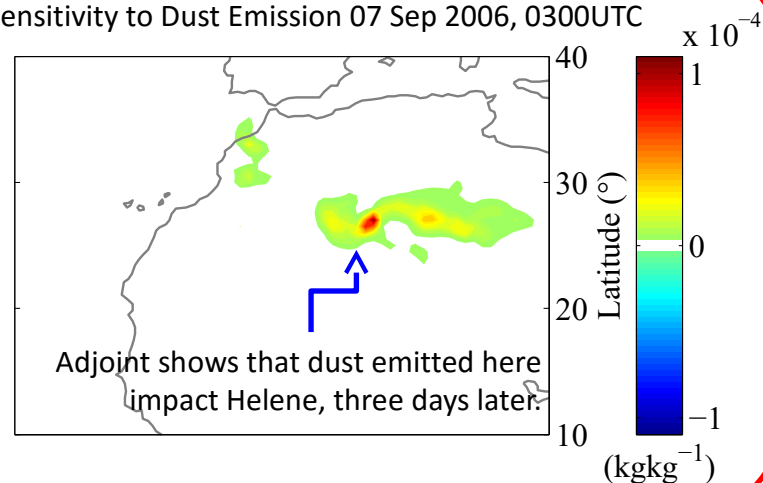
Sensitivity to Dust Emission 07 Sep 2006, 0300UTC
