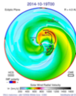
Computer model of the CME traveling through the solar system.
